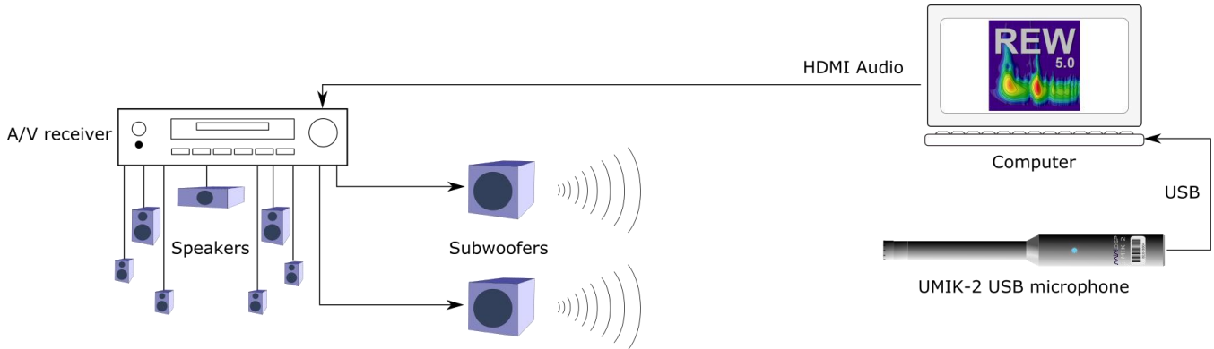
Figure 2. Typical measurement setup for REW
